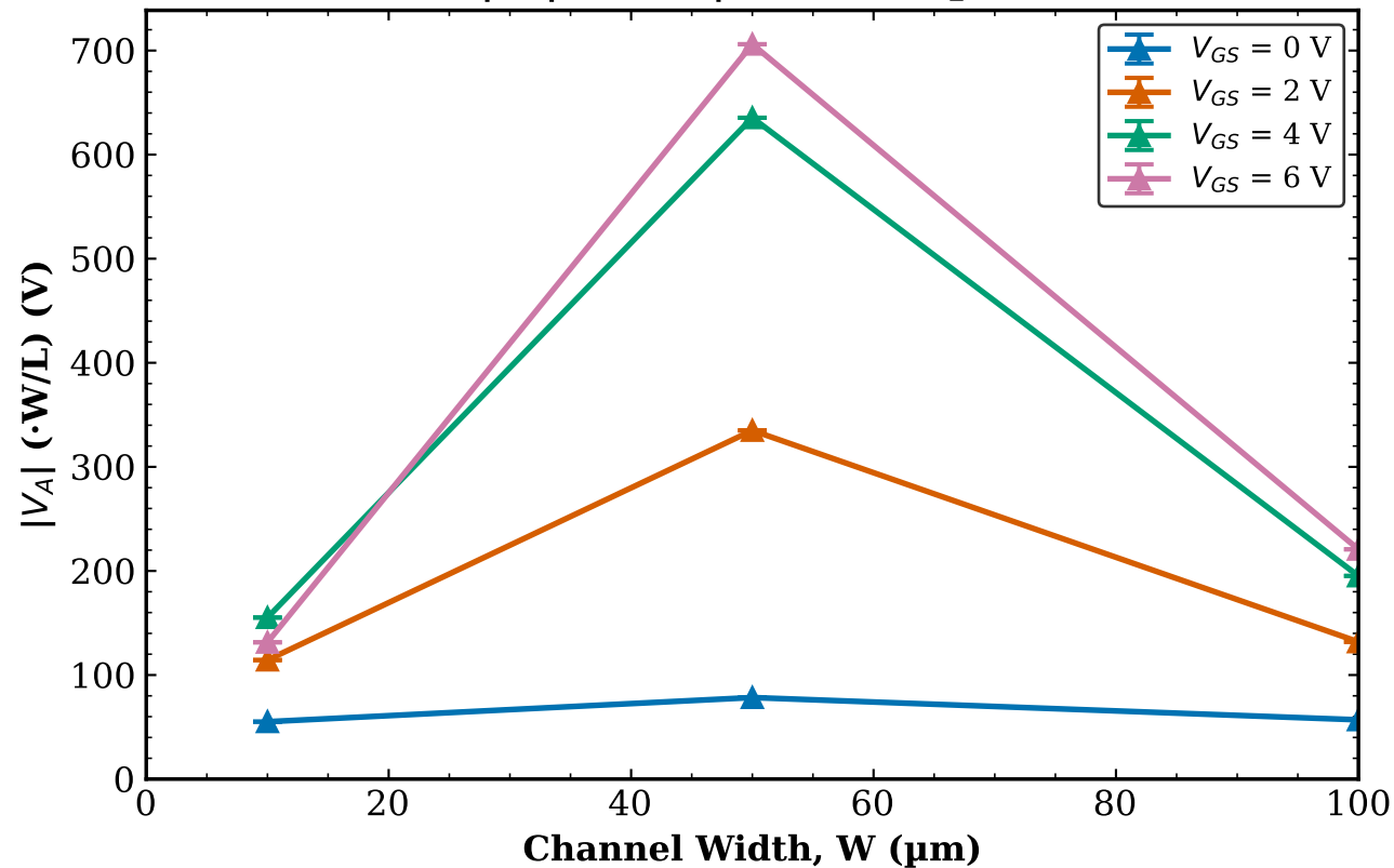
TFT1 Transistor 1 |V_A| vs W | L = 160\text{ }\mu\text{m}
